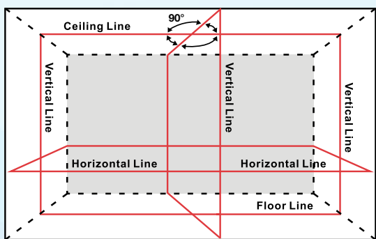
Showing ALL visual beams of the Tommi LR 430HDV
